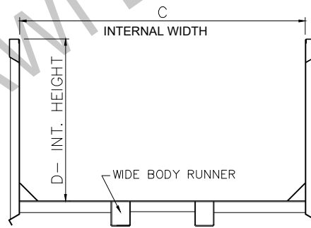
SECTIONAL VIEW
